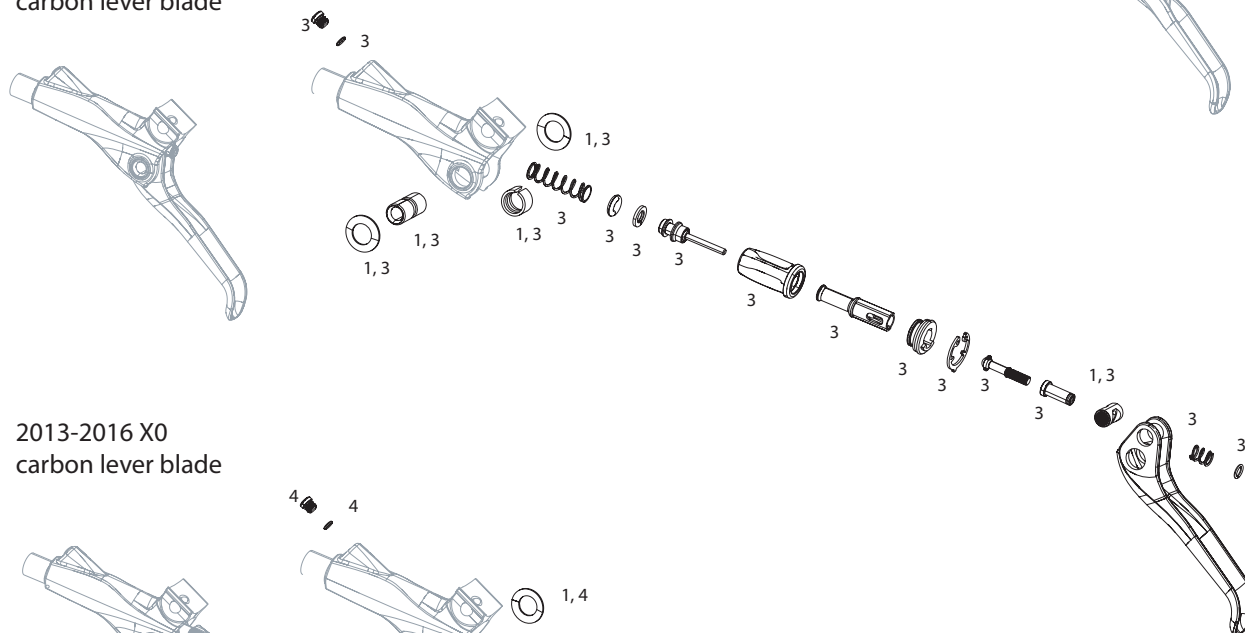
2013-2016 X0 GS (GripShift-compatible) carbon lever blade
